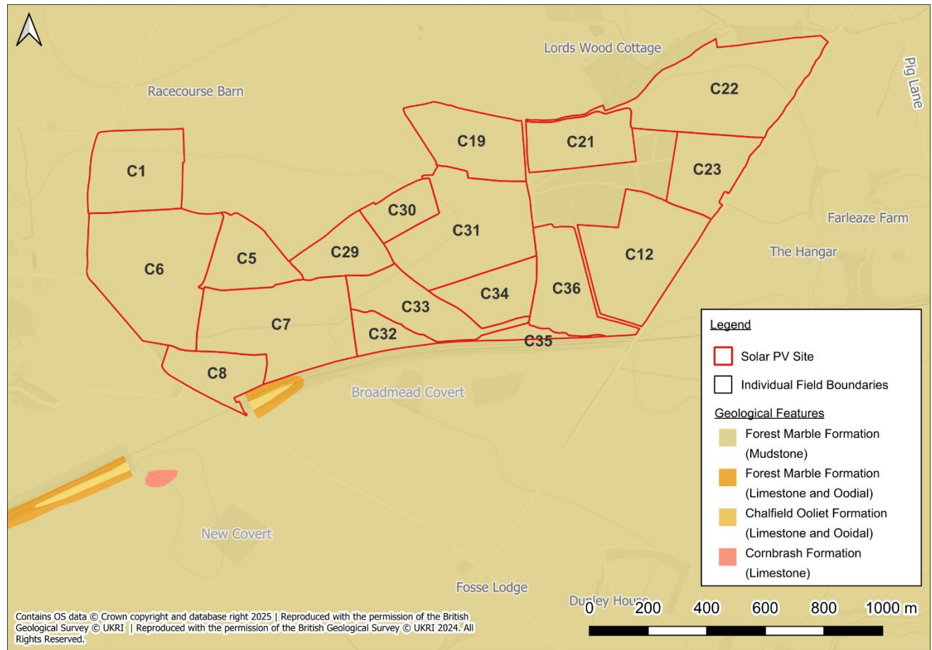
Figure 4: Bedrock Deposits
